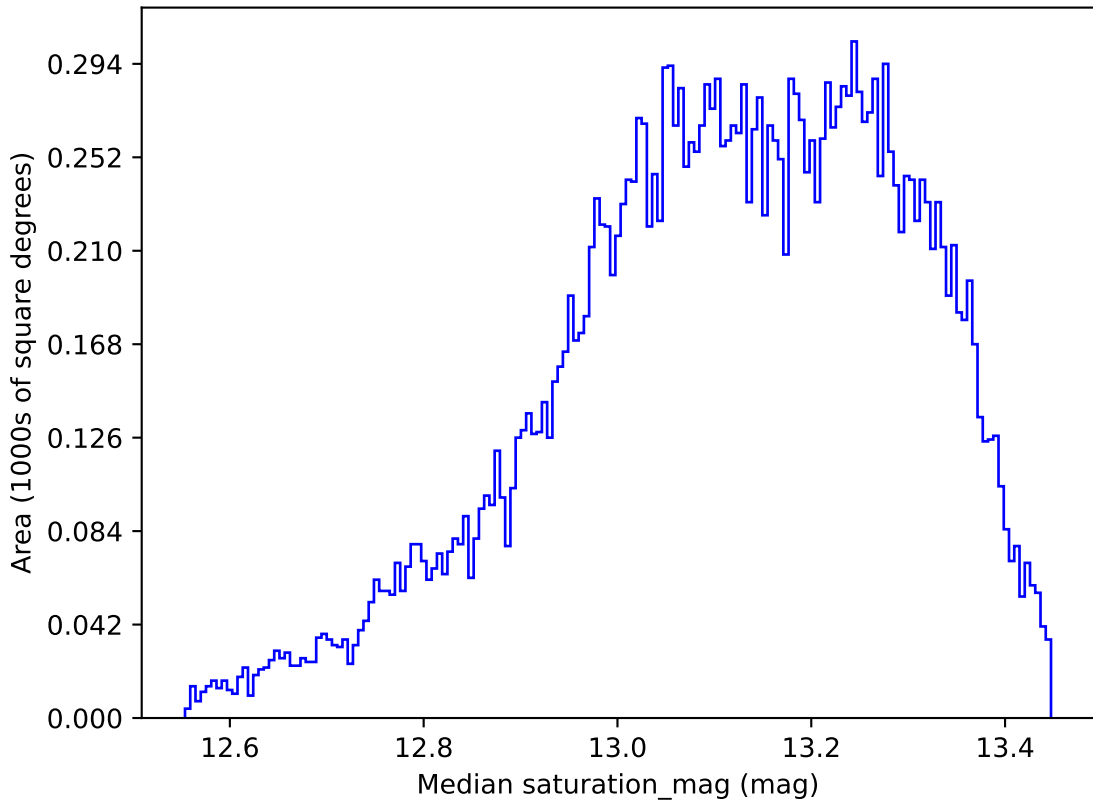
ddf_loaded_half_fl8_v3.4_10yrs All sky y band: Median saturation_mag
