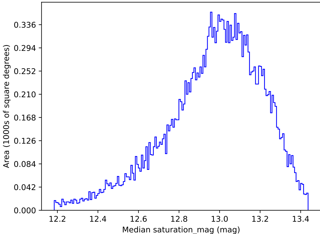
ddf_loaded_half_fl8_v3.4_10yrs All sky u band: Median saturation_mag
