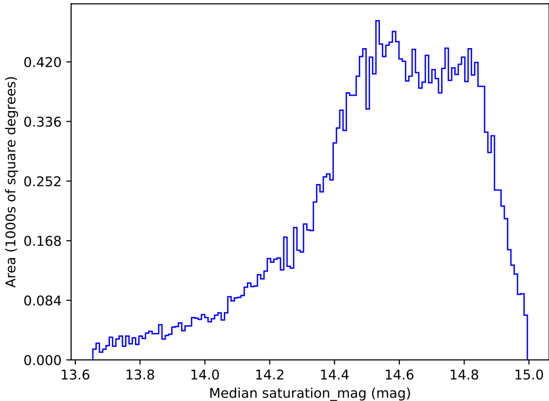
ddf_loaded_half_fl8_v3.4_10yrs All sky r band: Median saturation_mag
