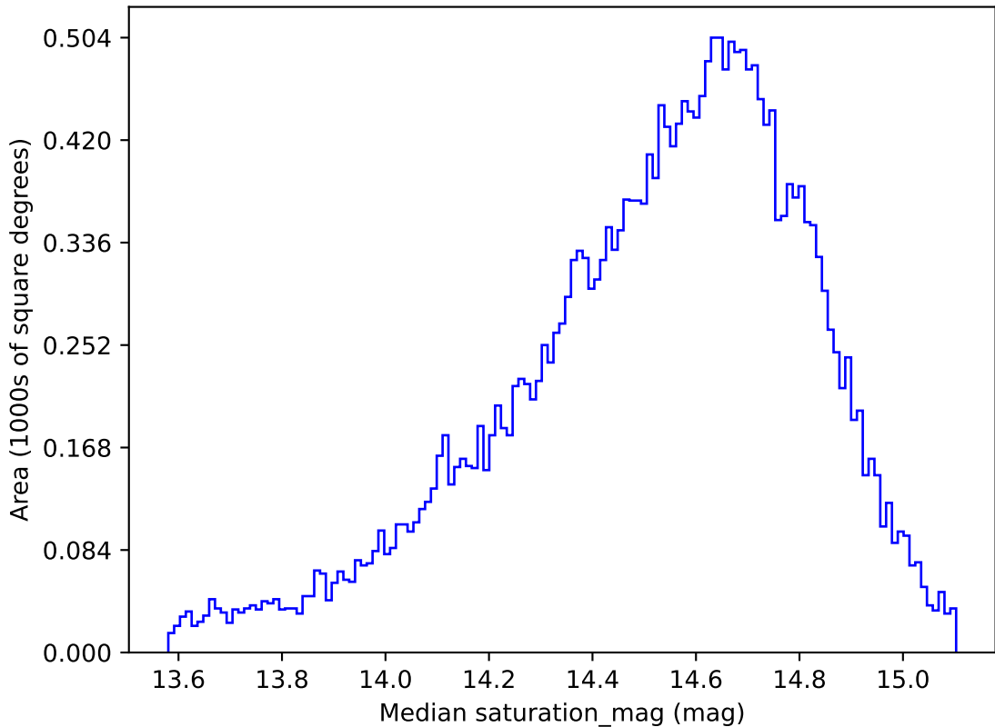
ddf_loaded_half_fl8_v3.4_10yrs All sky g band: Median saturation_mag
