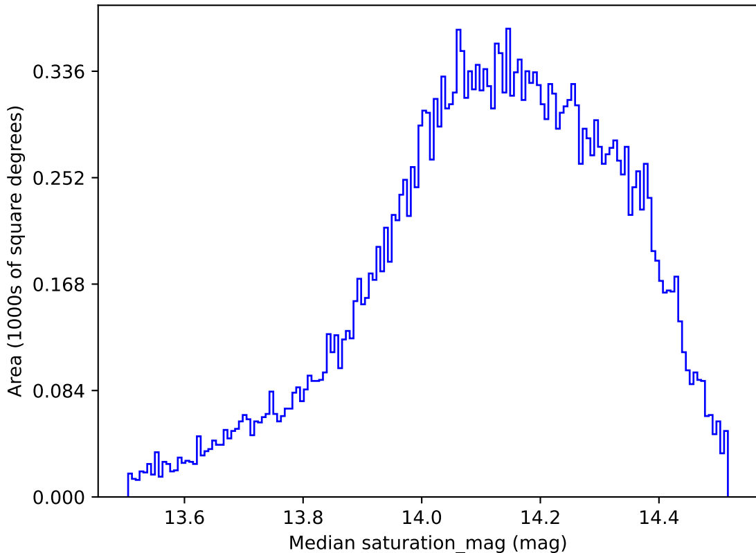
ddf_loaded_half_fl8_v3.4_10yrs All sky all bands: Median saturation_mag
