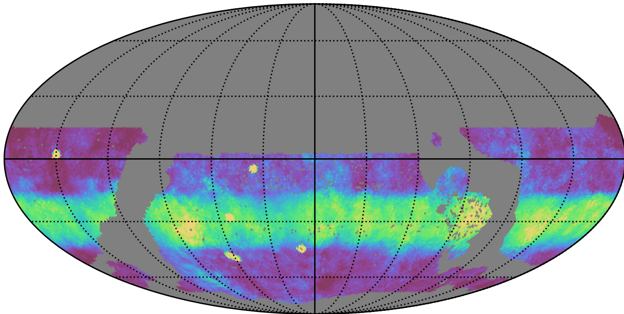
ddf_loaded_half_fl8_v3.4_10yrs WFD y band: Median normairmass
