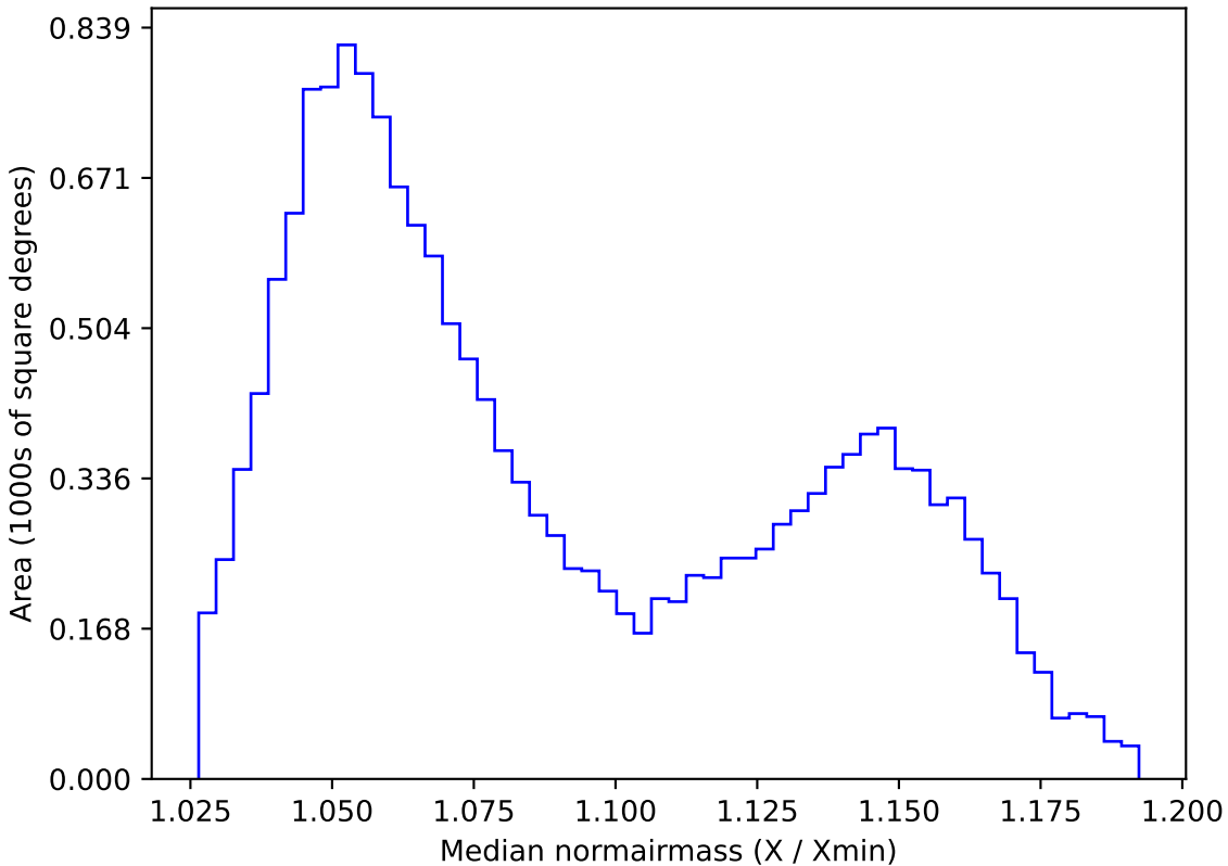
ddf_loaded_half_fl8_v3.4_10yrs WFD y band: Median normairmass
