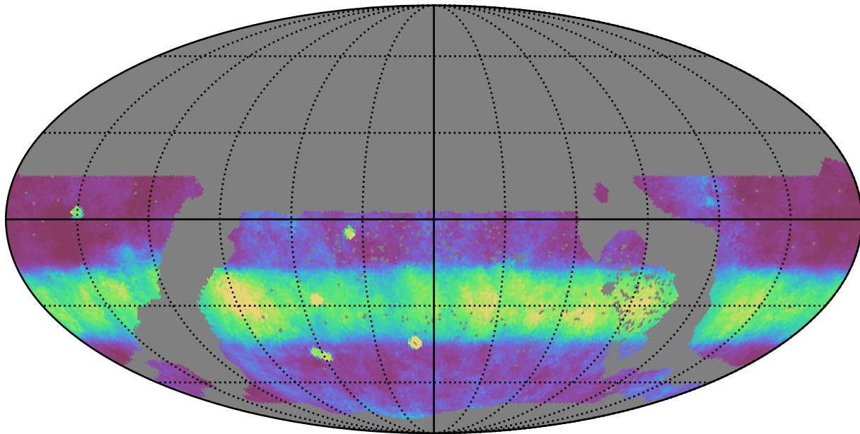
ddf_loaded_half_fl8_v3.4_10yrs WFD r band: Median normairmass
