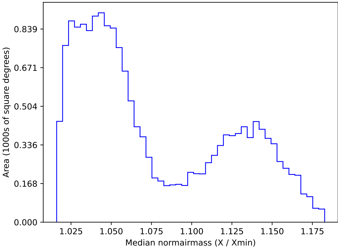
ddf_loaded_half_fl8_v3.4_10yrs WFD r band: Median normairmass
