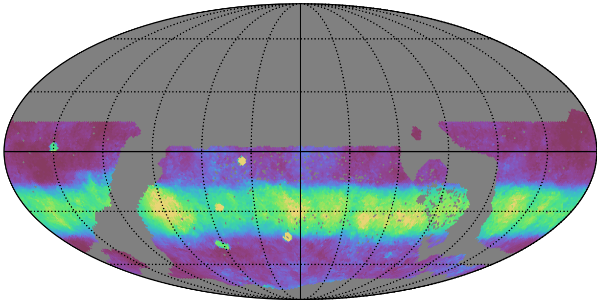
ddf_loaded_half_fl8_v3.4_10yrs WFD i band: Median normairmass
