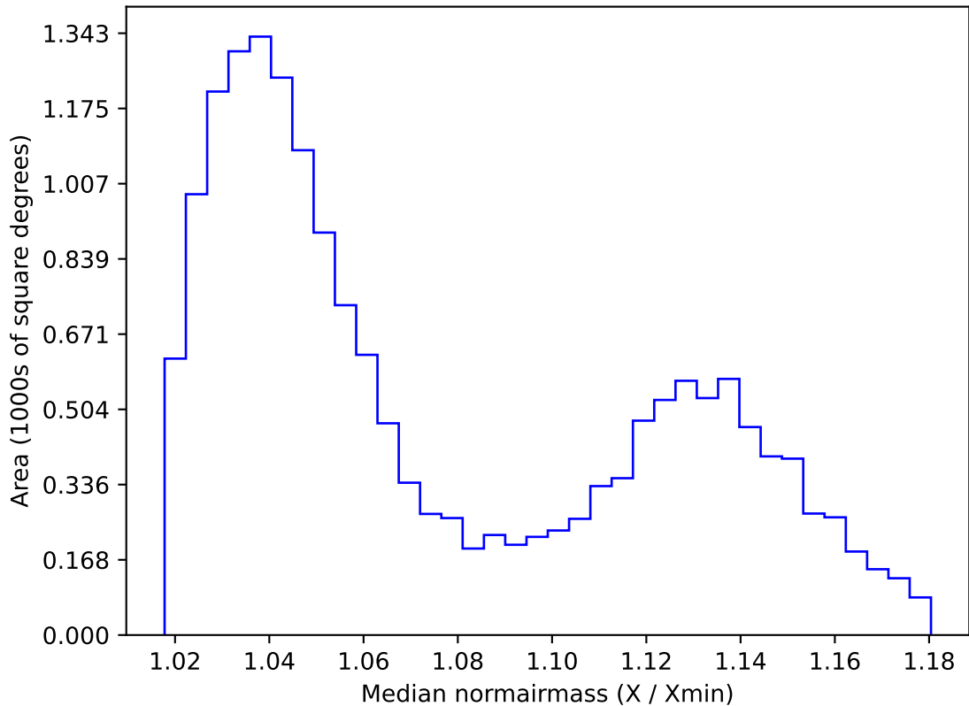
ddf_loaded_half_fl8_v3.4_10yrs WFD i band: Median normairmass
