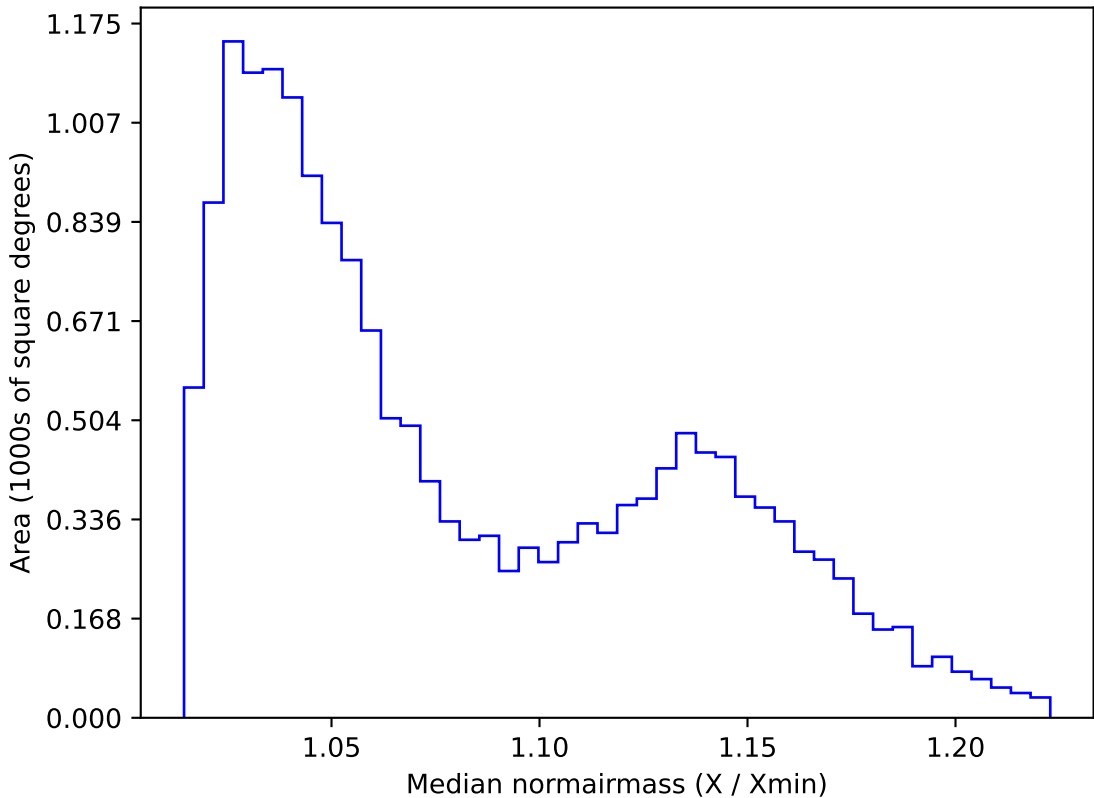
ddf_loaded_half_fl8_v3.4_10yrs WFD g band: Median normairmass
