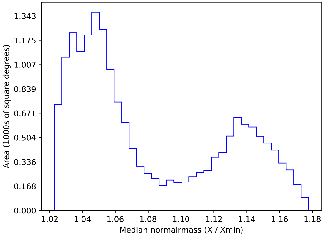
ddf_loaded_half_fl8_v3.4_10yrs WFD all bands: Median normairmass
