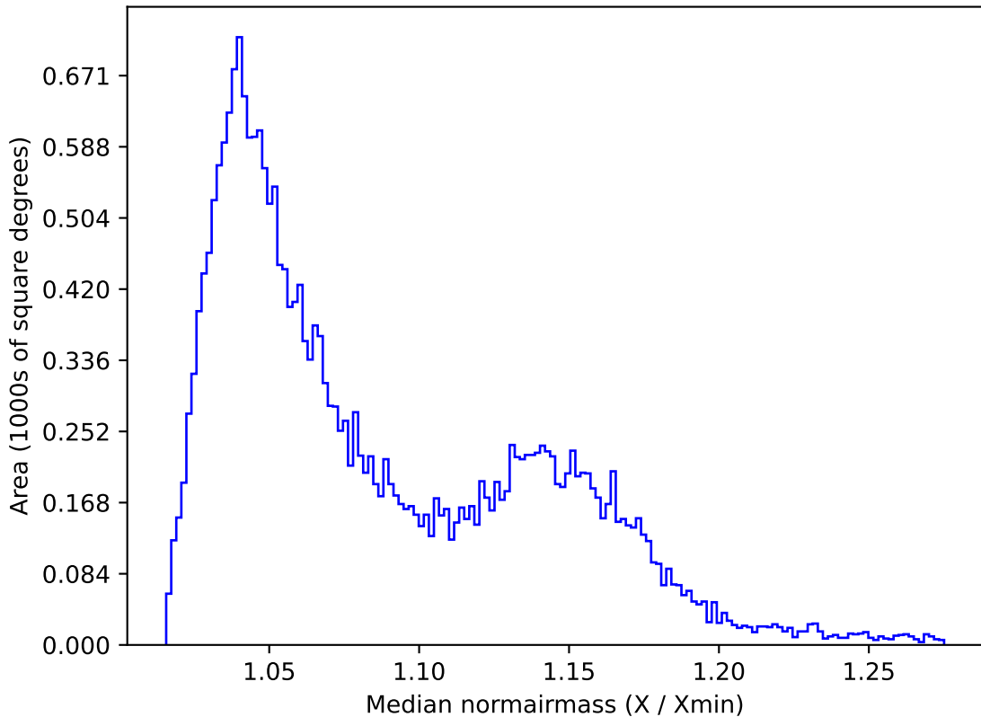
ddf_loaded_half_fl8_v3.4_10yrs All sky z band: Median normairmass
