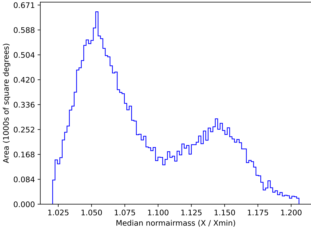
ddf_loaded_half_fl8_v3.4_10yrs All sky y band: Median normairmass
