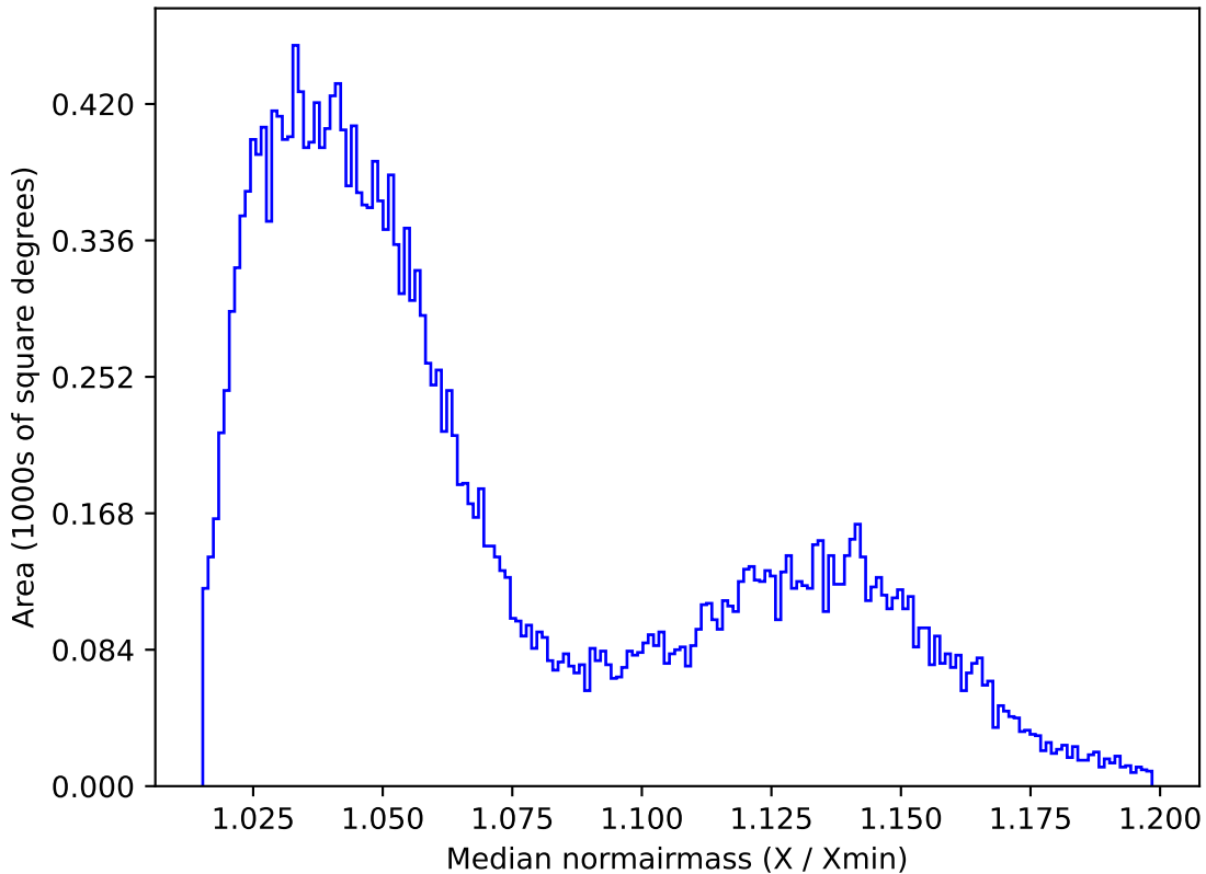
ddf_loaded_half_fl8_v3.4_10yrs All sky r band: Median normairmass
