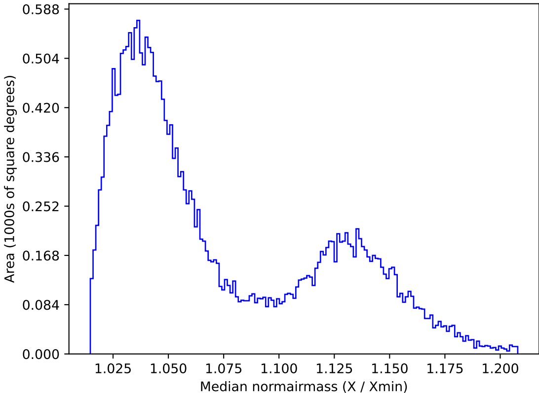
ddf_loaded_half_fl8_v3.4_10yrs All sky i band: Median normairmass
