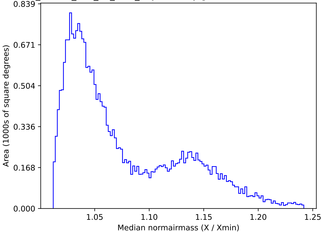
ddf_loaded_half_fl8_v3.4_10yrs All sky g band: Median normairmass
