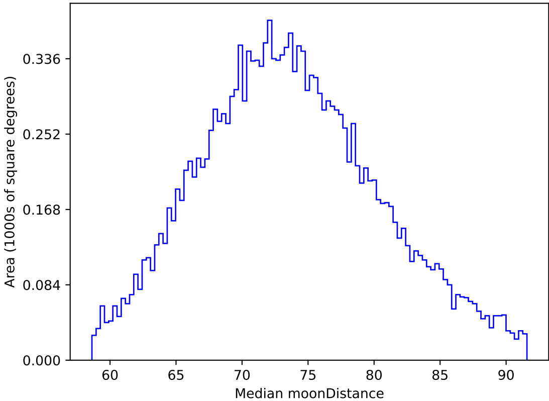
ddf_loaded_half_fl8_v3.4_10yrs WFD z band: Median moonDistance
