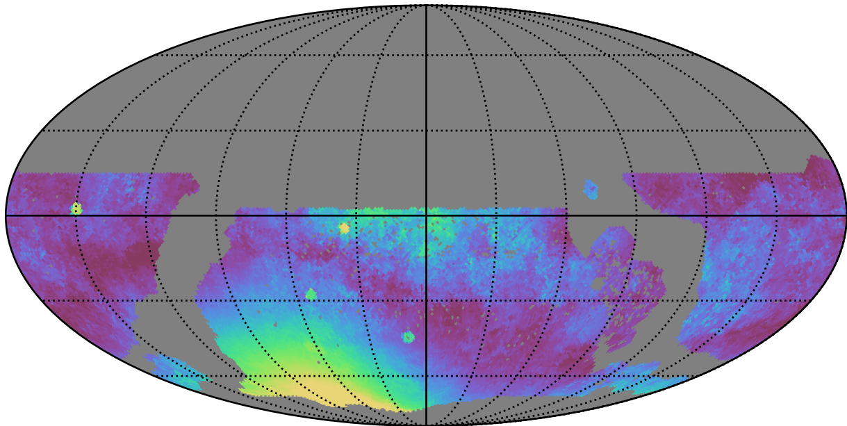
ddf_loaded_half_fl8_v3.4_10yrs WFD y band: Median moonDistance
