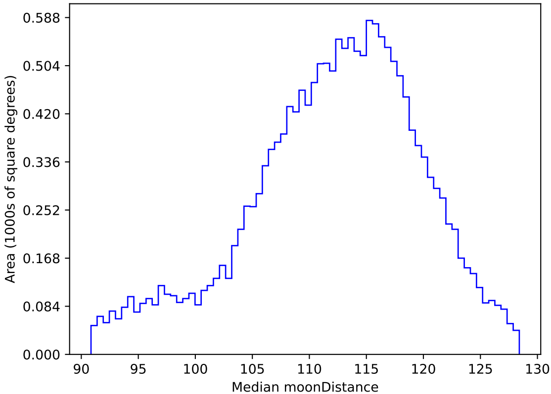
ddf_loaded_half_fl8_v3.4_10yrs WFD r band: Median moonDistance
