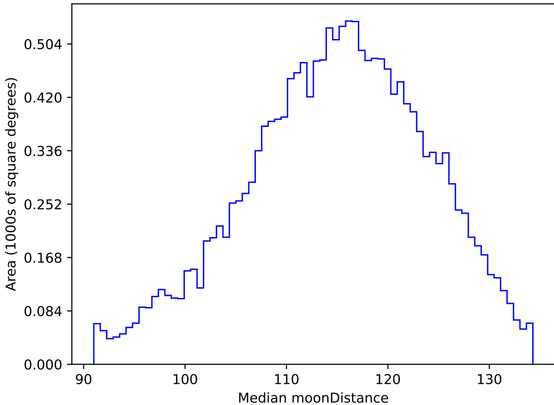
ddf_loaded_half_fl8_v3.4_10yrs WFD g band: Median moonDistance
