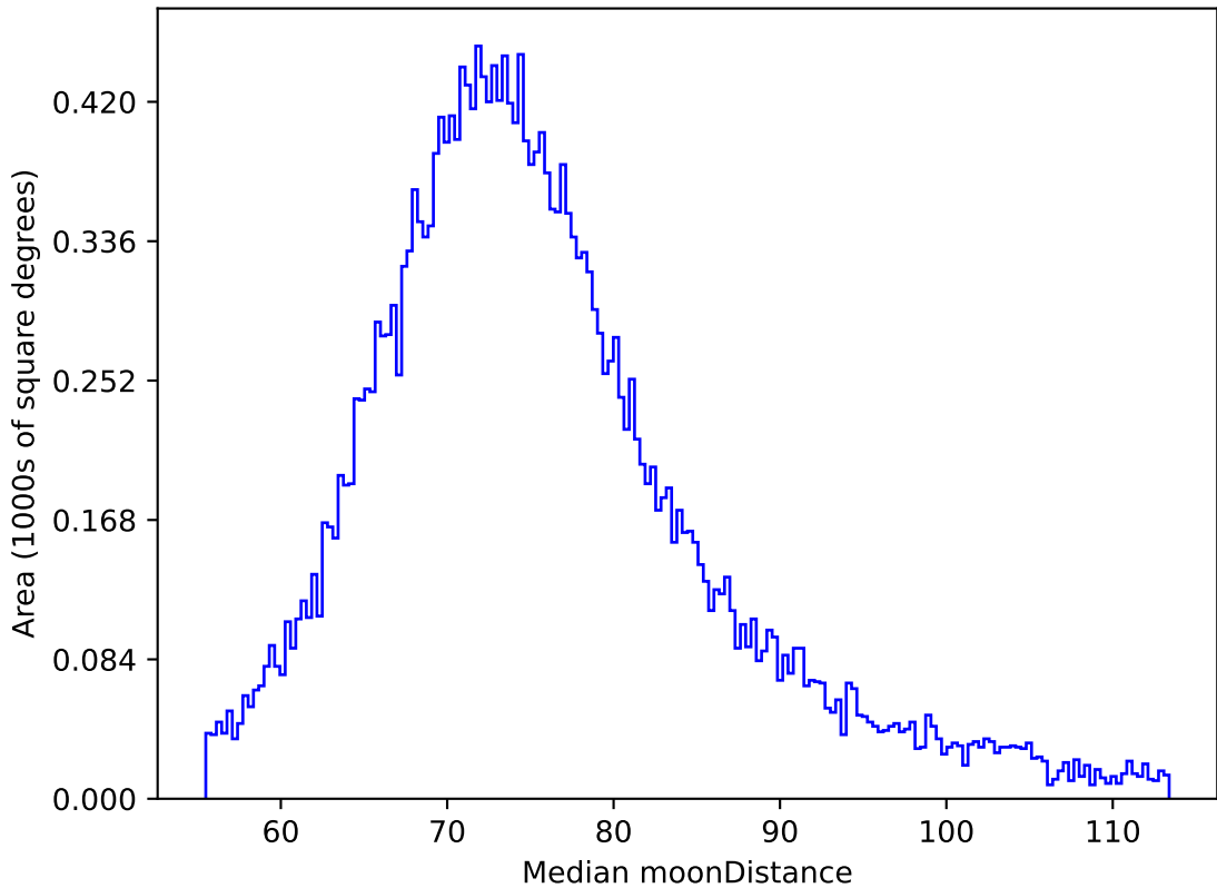
ddf_loaded_half_fl8_v3.4_10yrs All sky z band: Median moonDistance
