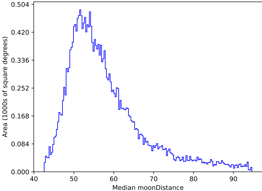
ddf_loaded_half_fl8_v3.4_10yrs All sky y band: Median moonDistance
