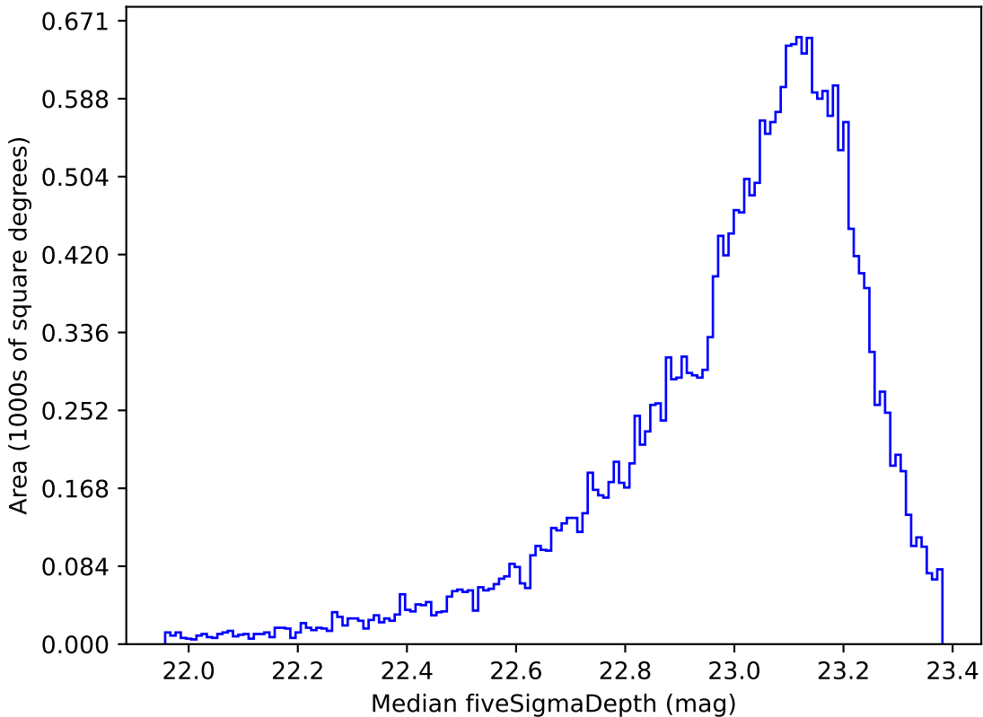
ddf_loaded_half_fl8_v3.4_10yrs Yr 1 z band: Median fiveSigmaDepth
