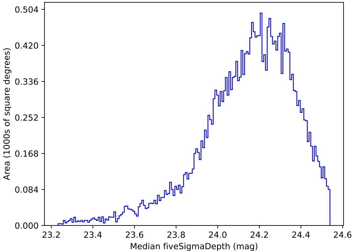
ddf_loaded_half_fl8_v3.4_10yrs Yr 1 r band: Median fiveSigmaDepth
