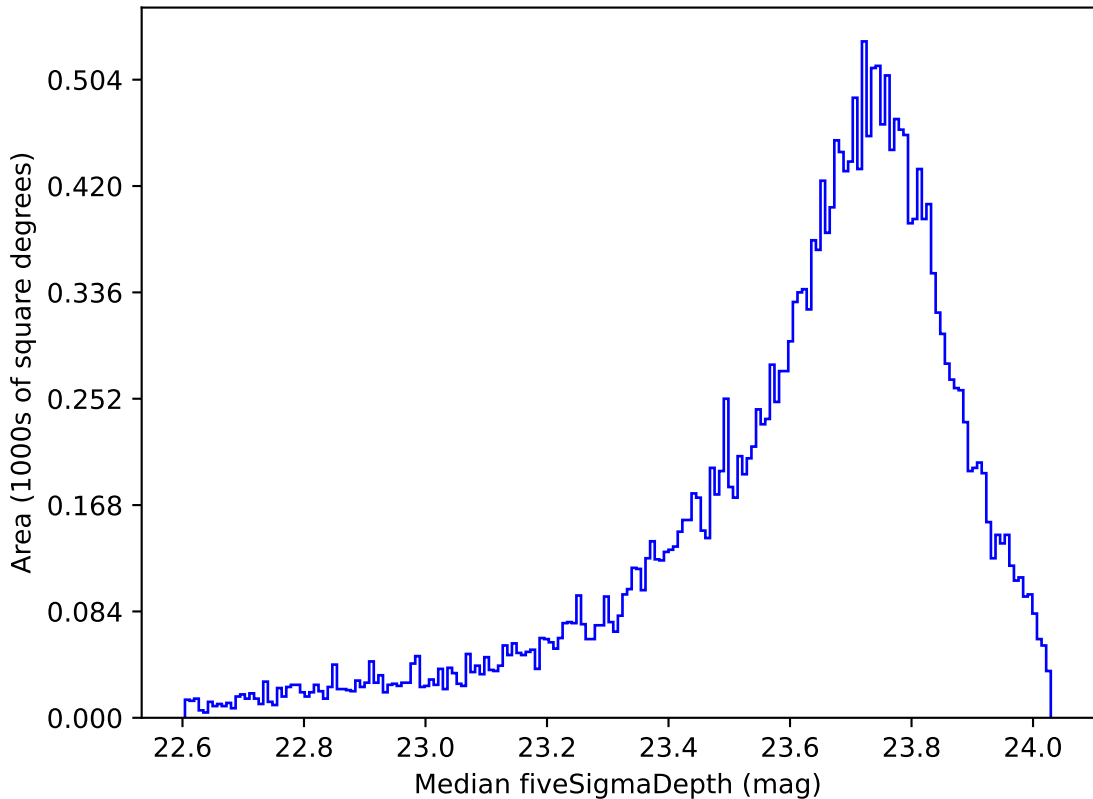
ddf_loaded_half_fl8_v3.4_10yrs Yr 1 i band: Median fiveSigmaDepth
