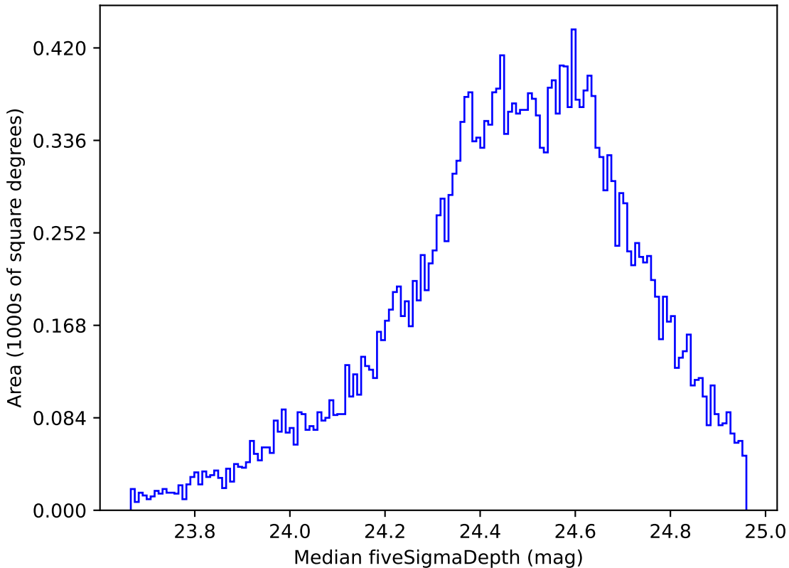
ddf_loaded_half_fl8_v3.4_10yrs Yr 1 g band: Median fiveSigmaDepth
