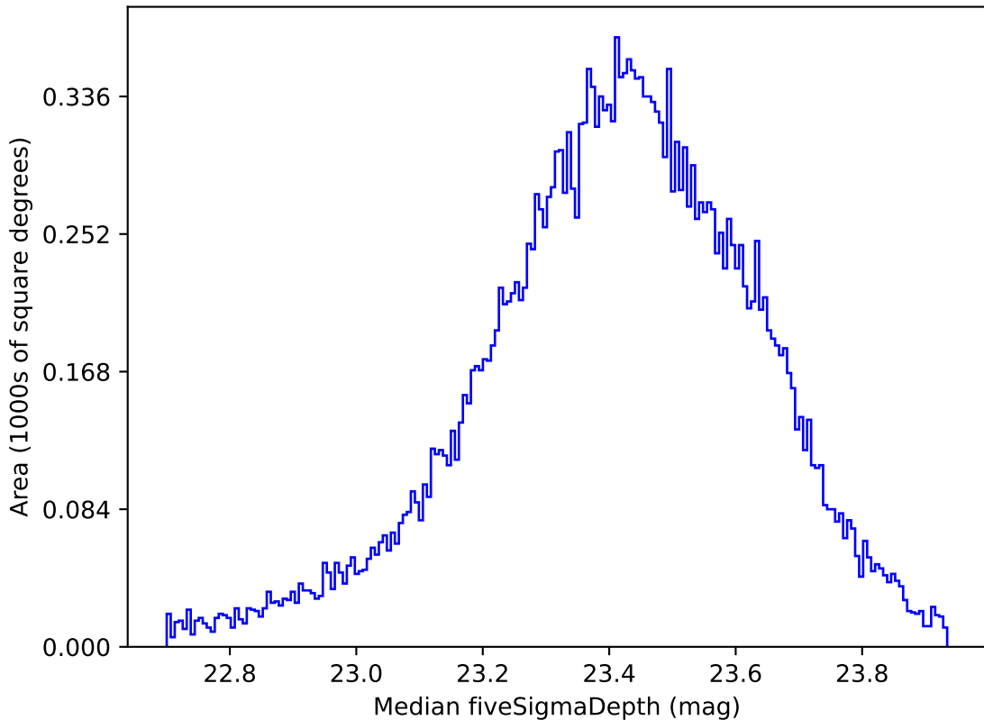
ddf_loaded_half_fl8_v3.4_10yrs Yr 1 all bands: Median fiveSigmaDepth
