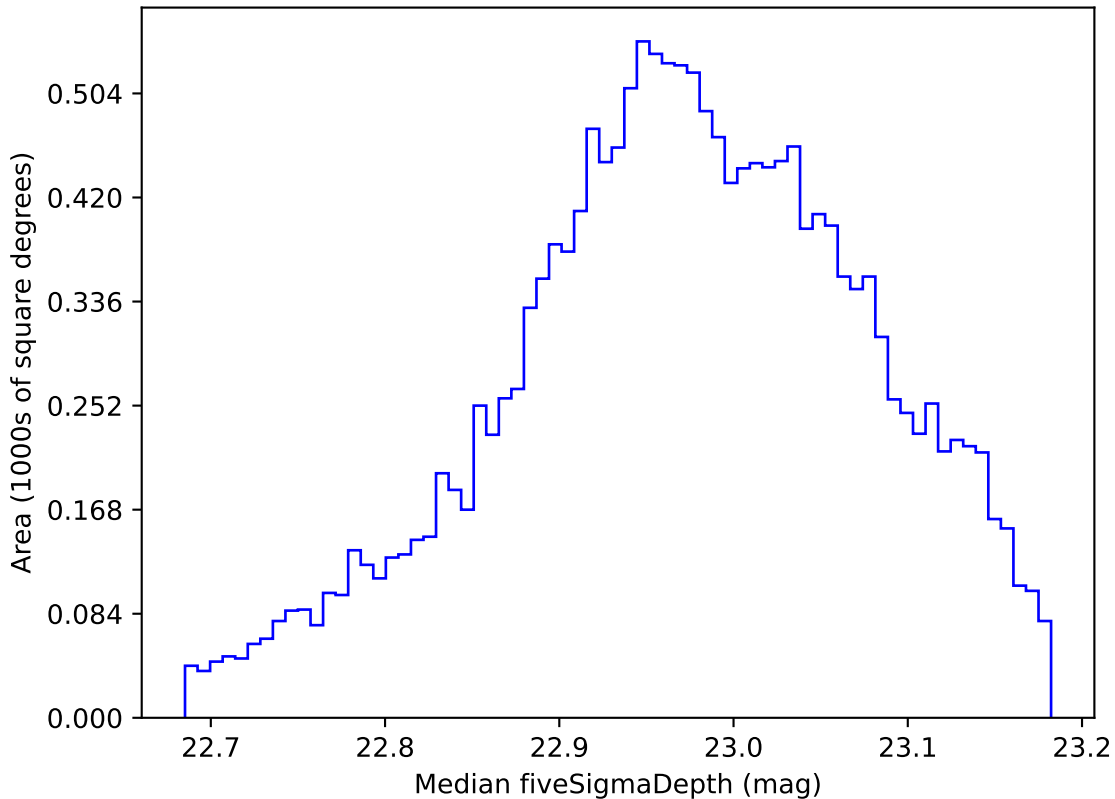
ddf_loaded_half_fl8_v3.4_10yrs WFD z band: Median fiveSigmaDepth
