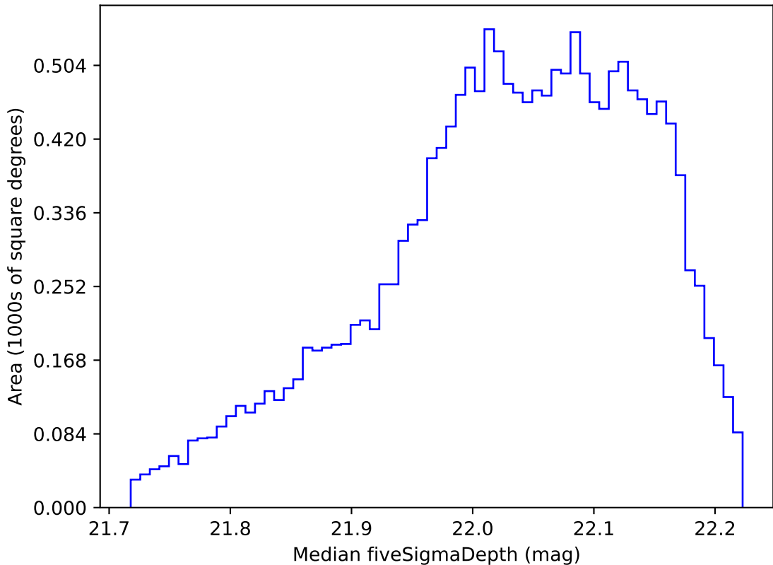
ddf_loaded_half_fl8_v3.4_10yrs WFD y band: Median fiveSigmaDepth
