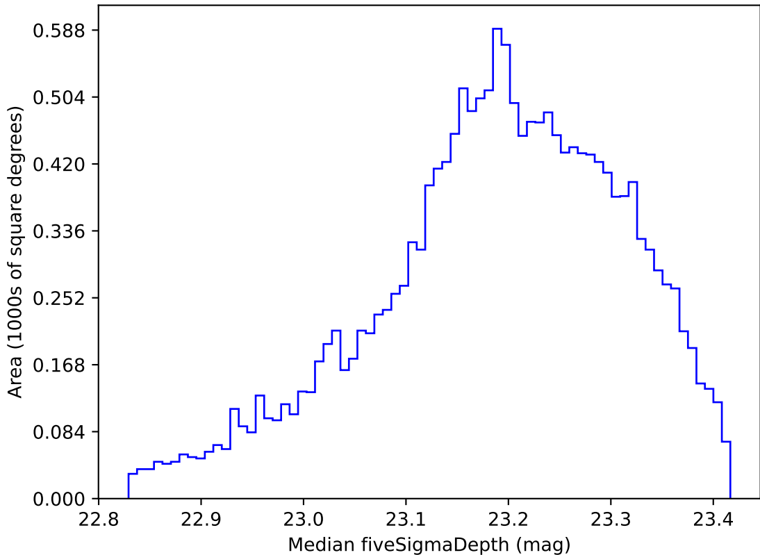
ddf_loaded_half_fl8_v3.4_10yrs WFD u band: Median fiveSigmaDepth
