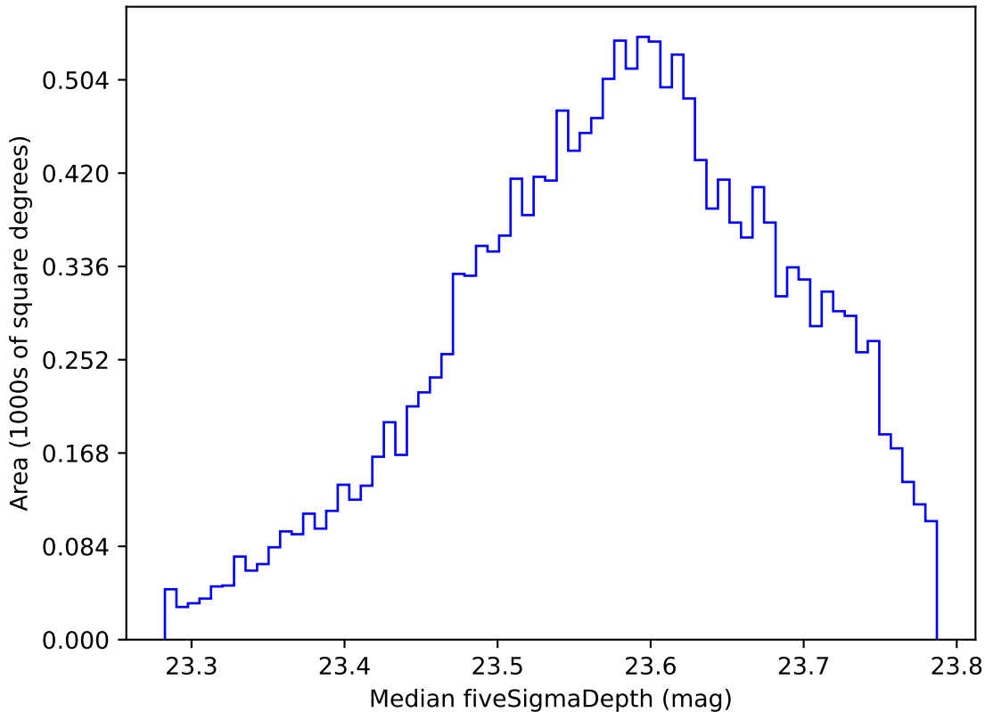
ddf_loaded_half_fl8_v3.4_10yrs WFD i band: Median fiveSigmaDepth
