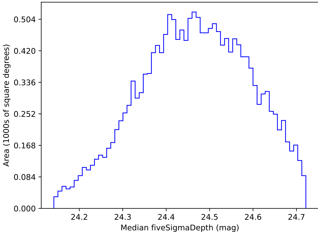
ddf_loaded_half_fl8_v3.4_10yrs WFD g band: Median fiveSigmaDepth
