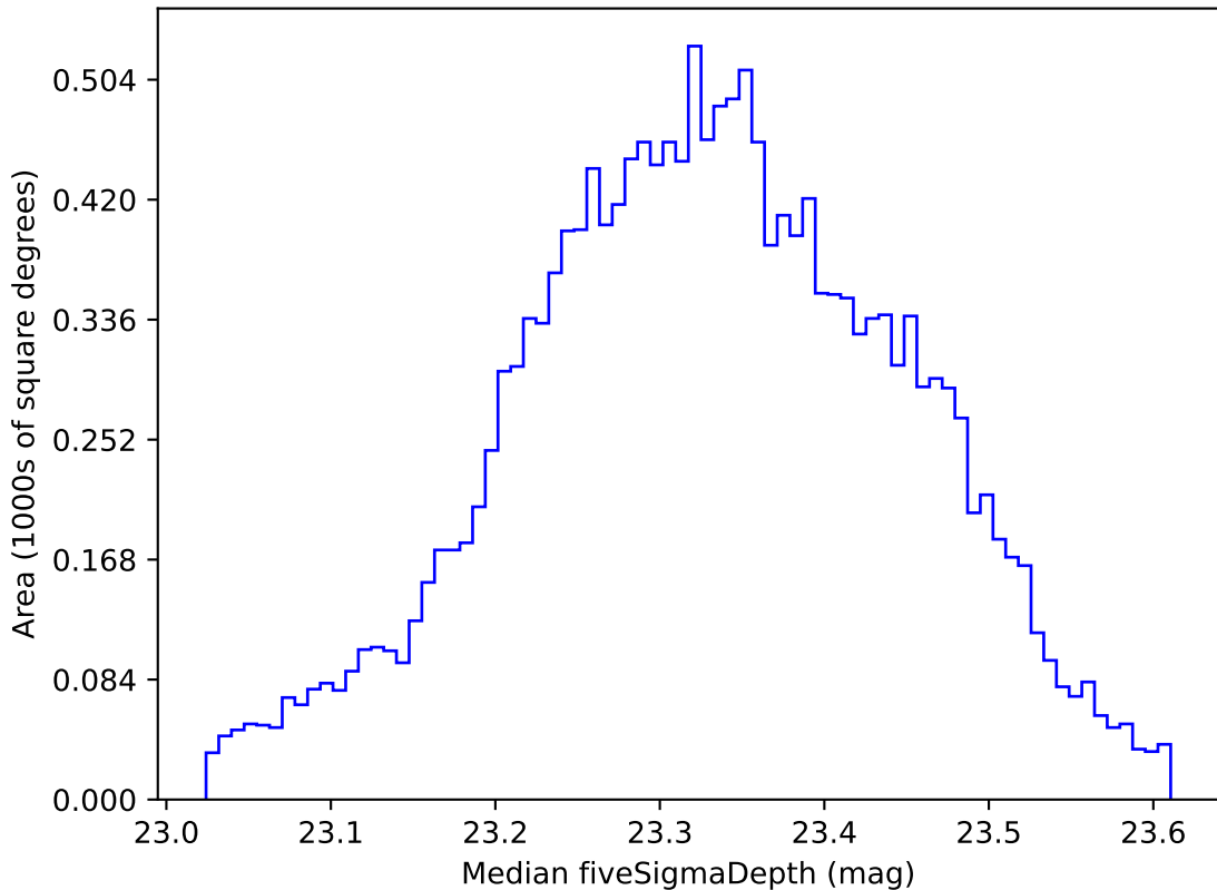
ddf_loaded_half_fl8_v3.4_10yrs WFD all bands: Median fiveSigmaDepth
