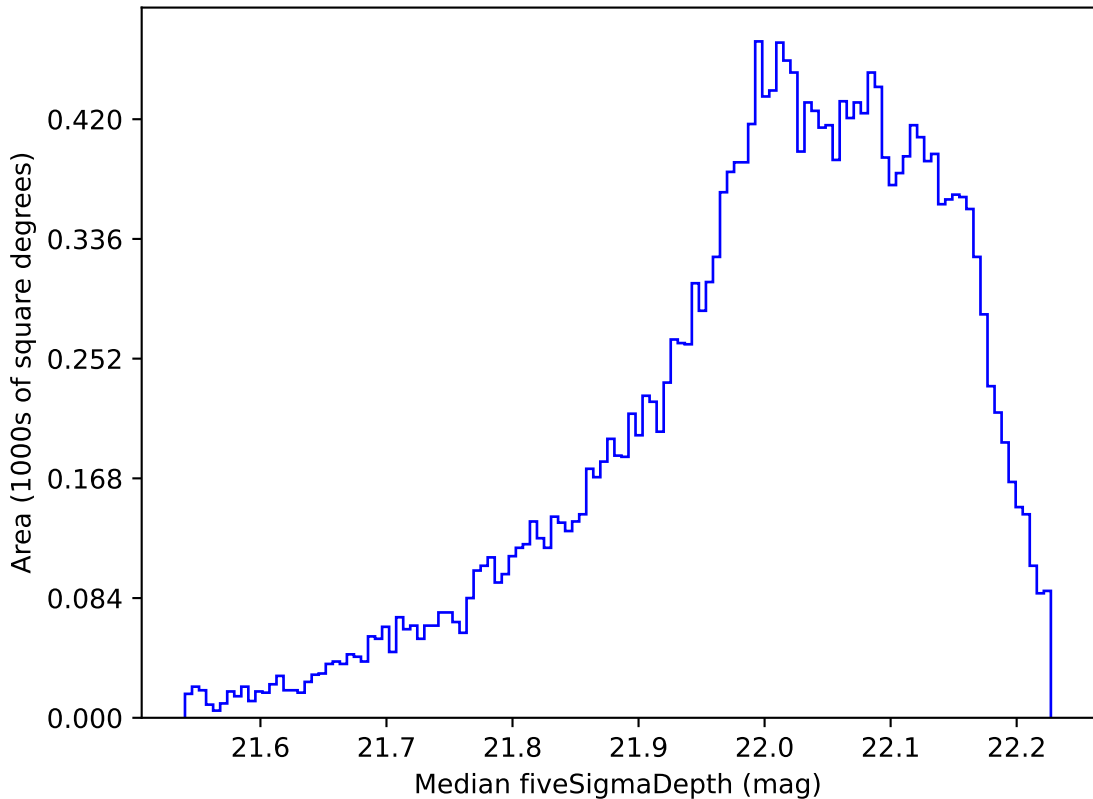
ddf_loaded_half_fl8_v3.4_10yrs All sky y band: Median fiveSigmaDepth
