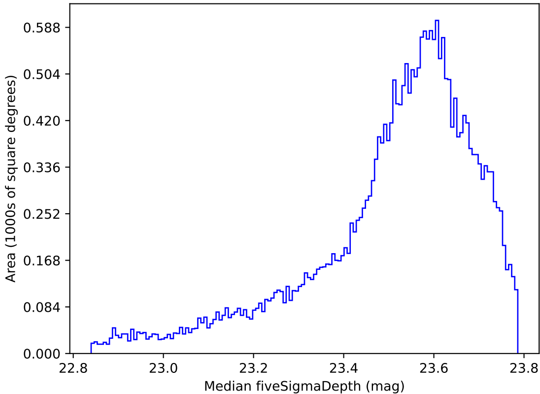
ddf_loaded_half_fl8_v3.4_10yrs All sky i band: Median fiveSigmaDepth
