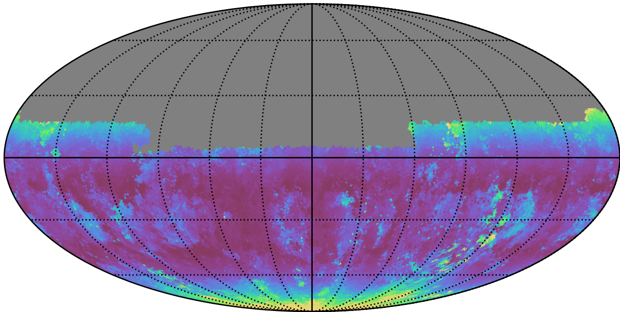
ddf_loaded_half_fl8_v3.4_10yrs Yr 1 u band: Median airmass
