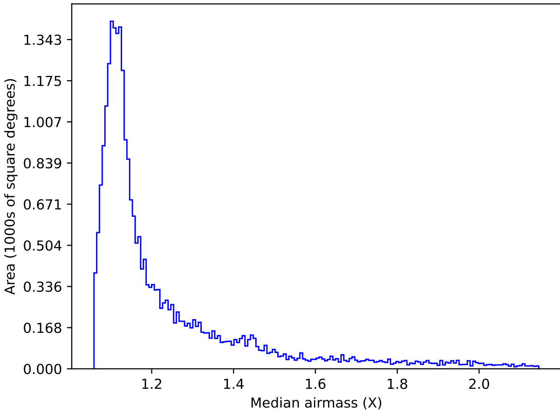
ddf_loaded_half_fl8_v3.4_10yrs Yr 1 i band: Median airmass
