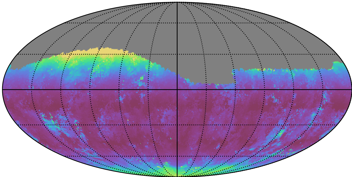
ddf_loaded_half_fl8_v3.4_10yrs Yr 1 g band: Median airmass
