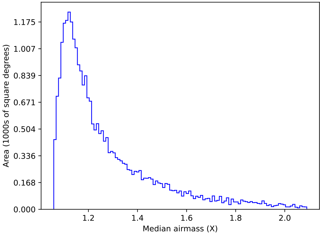
ddf_loaded_half_fl8_v3.4_10yrs Yr 1 g band: Median airmass
