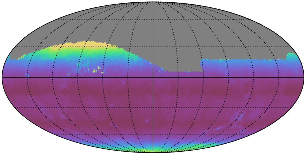
ddf_loaded_half_fl8_v3.4_10yrs Yr 1 all bands: Median airmass
