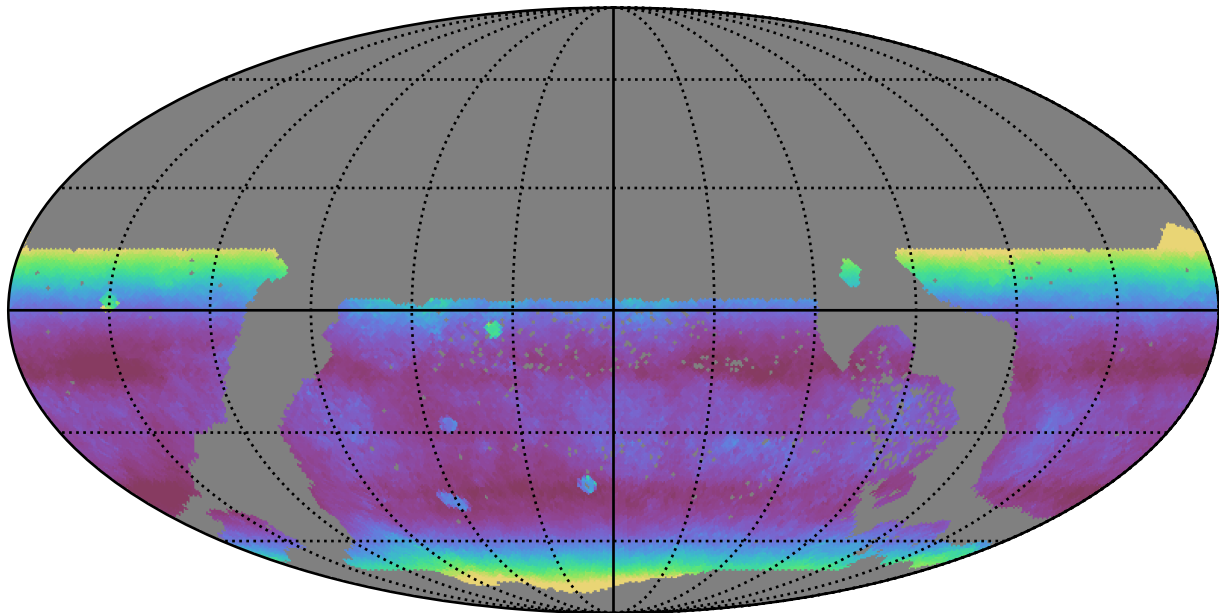
ddf_loaded_half_fl8_v3.4_10yrs WFD z band: Median airmass
