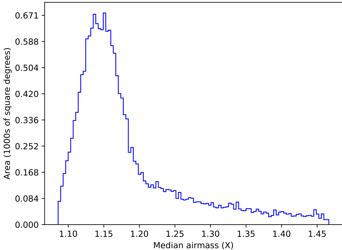
ddf_loaded_half_fl8_v3.4_10yrs WFD z band: Median airmass
