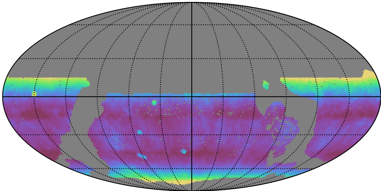
ddf_loaded_half_fl8_v3.4_10yrs WFD y band: Median airmass
