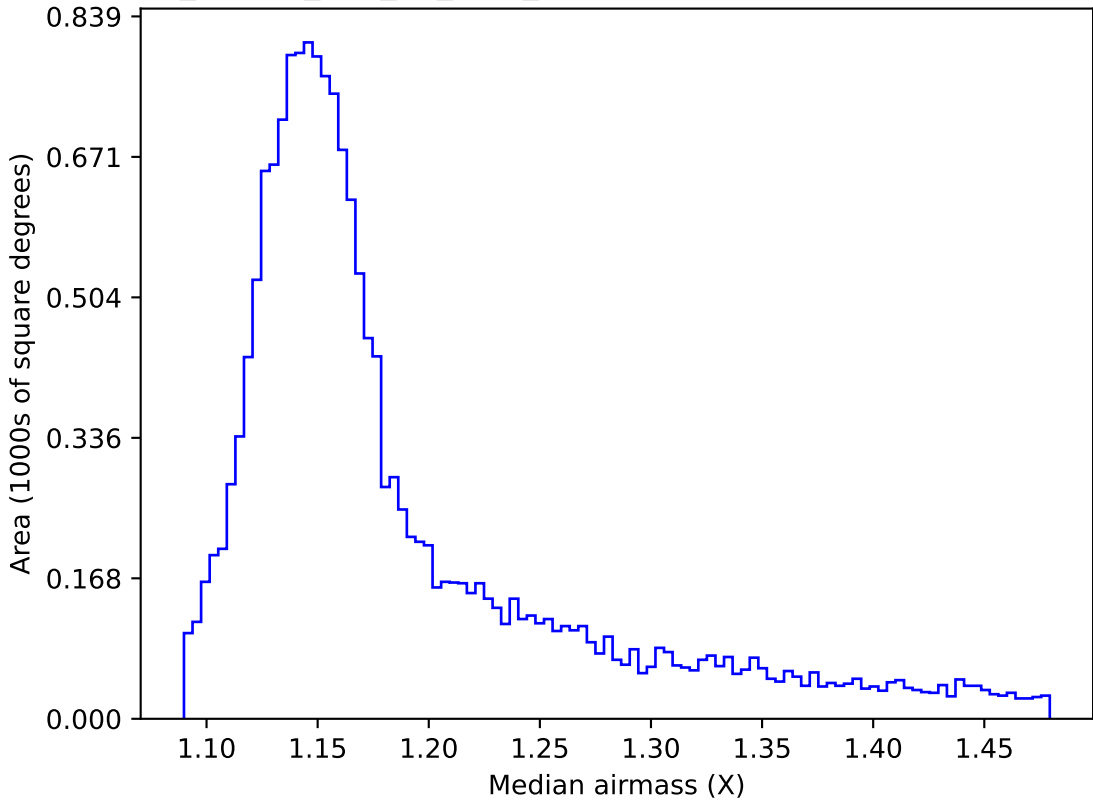
ddf_loaded_half_fl8_v3.4_10yrs WFD y band: Median airmass
