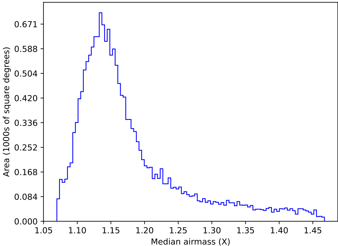
ddf_loaded_half_f18_v3.4_10yrs WFD u band: Median airmass
