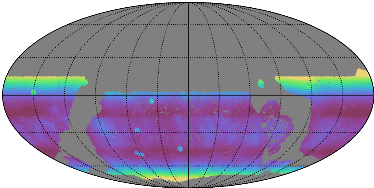
ddf_loaded_half_fl8_v3.4_10yrs WFD r band: Median airmass
