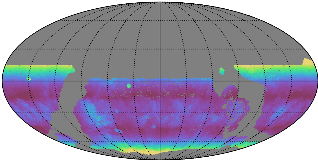
ddf_loaded_half_fl8_v3.4_10yrs WFD g band: Median airmass
