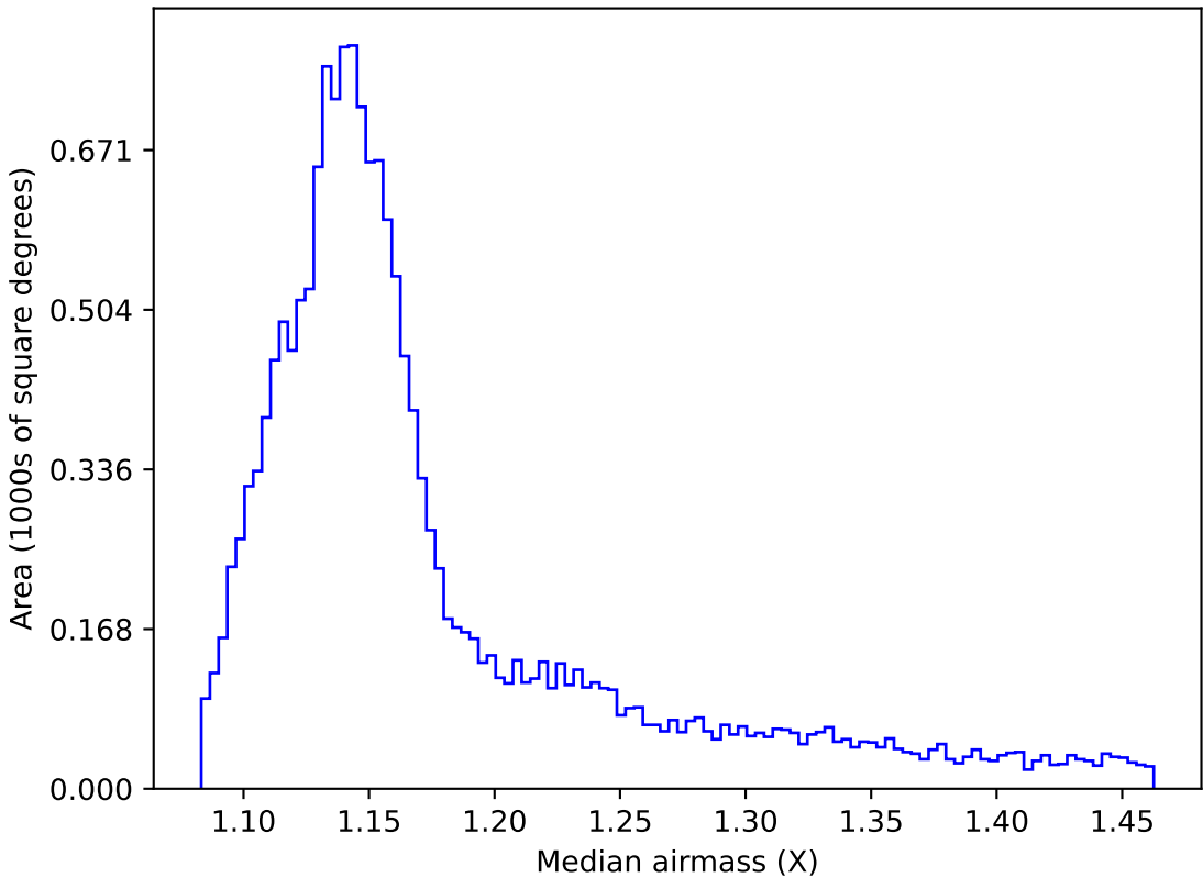
ddf_loaded_half_fl8_v3.4_10yrs WFD all bands: Median airmass
